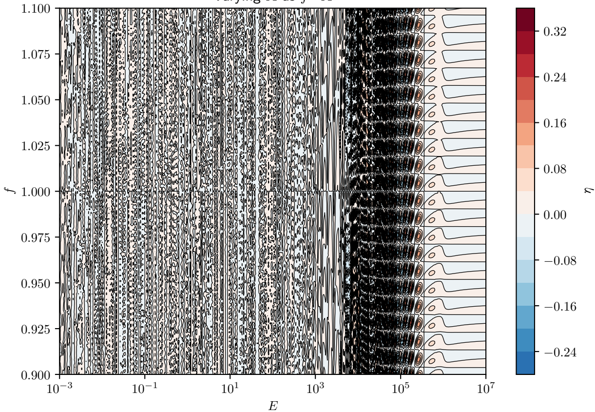
Relative P_{\mu\mu} variation for 'sun' model (passed through by 0.1 angle) Varying A as f \cdot A
