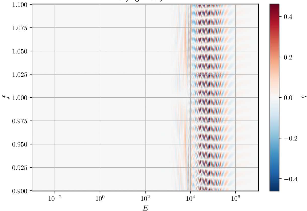
Relative P_{e\mu} variation for 'sun' model (passed through by 0.1 angle) Varying A as f \cdot A
