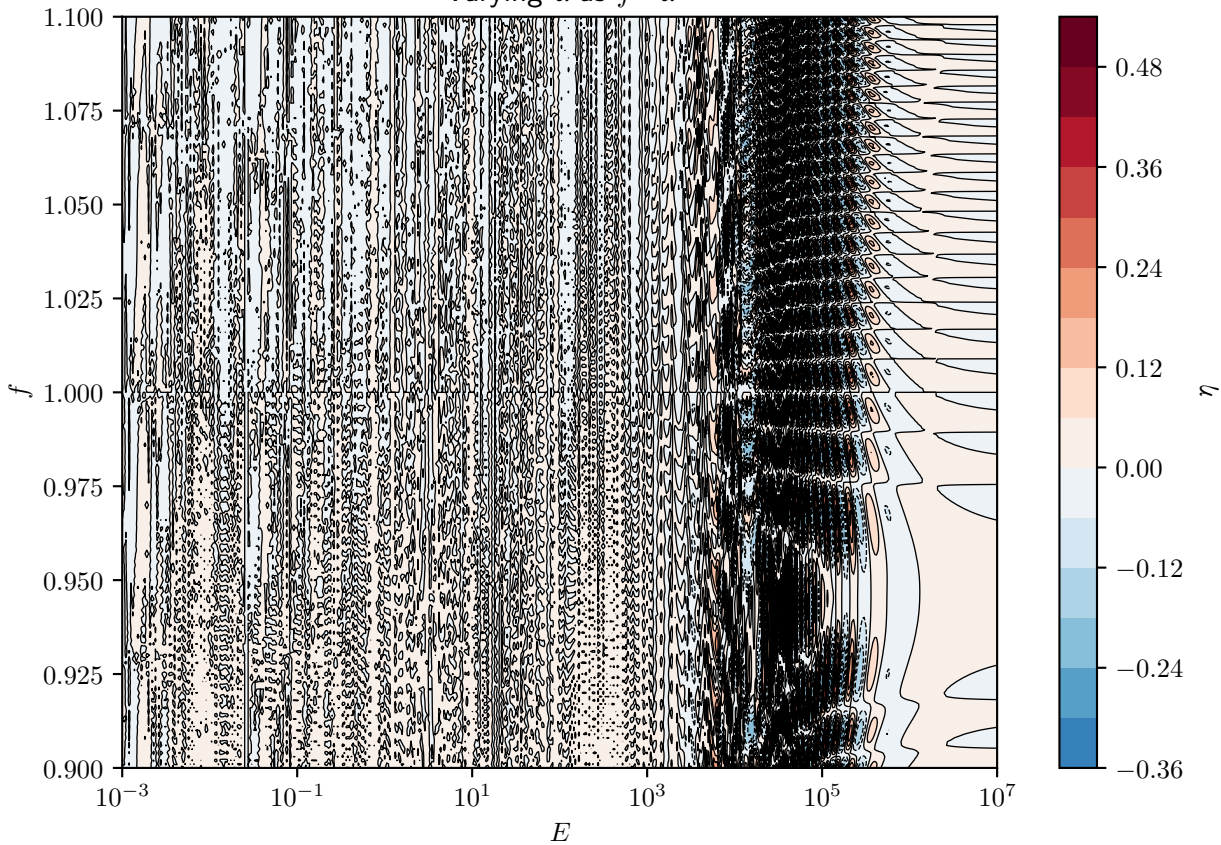
Relative P_{\text{eq}} variation for 'sun' model (passed through by 0.1 angle) Varying \alpha as f \cdot \alpha
