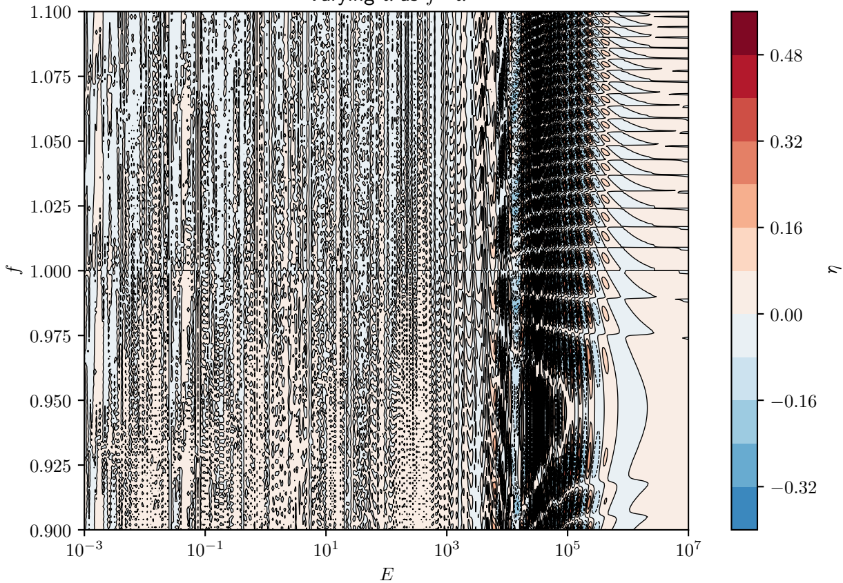
Relative P_{\text{eu}} variation for 'sun' model (passed through by 0.5 angle) Varying \alpha as f \cdot \alpha
