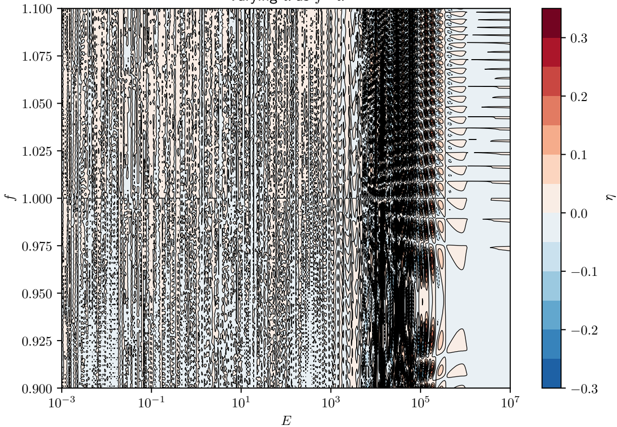
Relative P_{\mu\mu} variation for 'sun' model (passed through by 0.5 angle) Varying \alpha as f \cdot \alpha
