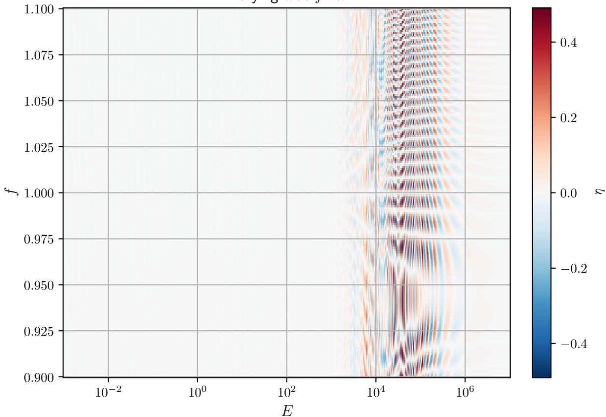
Relative P_{e\mu} variation for 'sun' model (passed through by 0.1 angle) Varying \alpha as f \cdot \alpha
