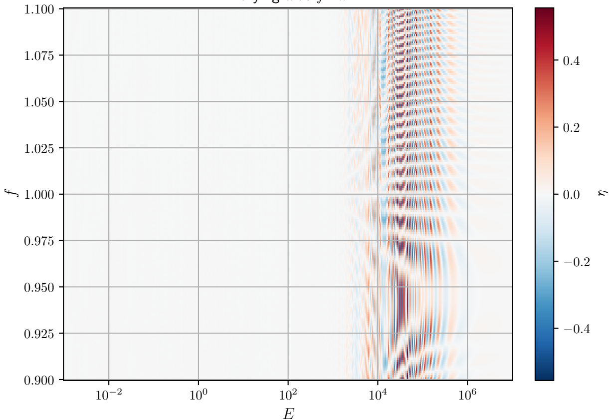
Relative P_{e\mu} variation for 'sun' model (passed through by 0.5 angle) Varying \alpha as f \cdot \alpha
