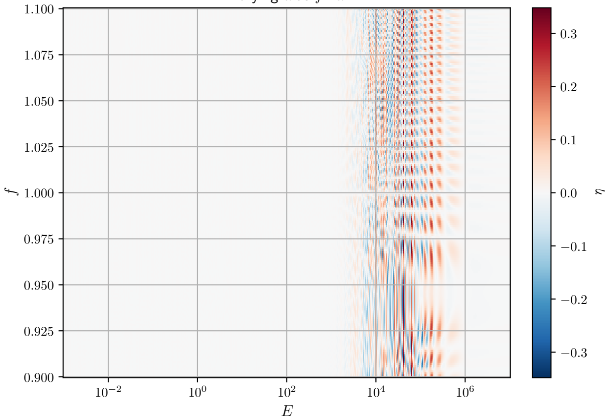
Relative P_{\mu\mu} variation for 'sun' model (passed through by 0.1 angle) Varying \alpha as f \cdot \alpha
