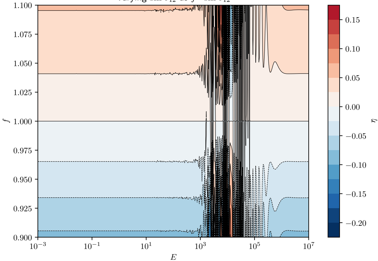
Relative P_{\text{e}\mu} variation for 'sun' model (passed through by 0.1 angle) Varying \sin \vartheta_{12} as f \cdot \sin \vartheta_{12}
