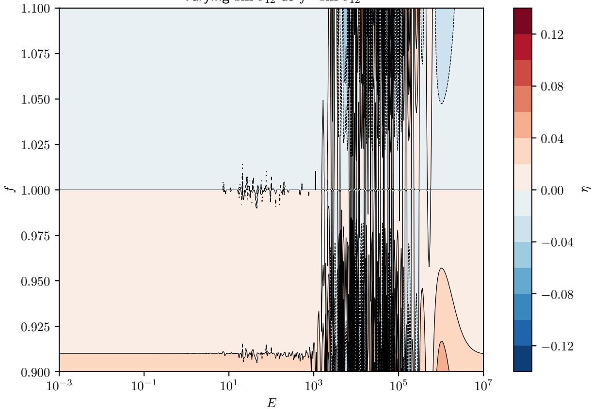
Relative P_{\mu\mu} variation for 'sun' model (passed through by 0.1 angle) Varying \sin \vartheta_{12} as f \cdot \sin \vartheta_{12}
