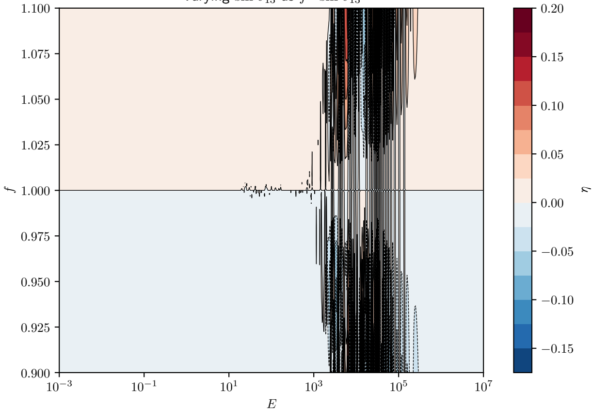
Relative P_{\text{e}\mu} variation for 'sun' model (passed through by 0.1 angle) Varying \sin \vartheta_{13} as f \cdot \sin \vartheta_{13}
