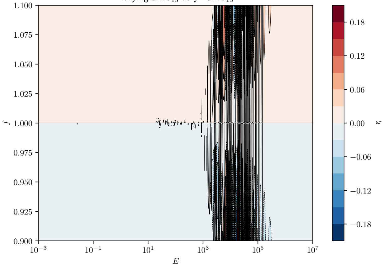
Relative P_{\text{e}\mu} variation for 'sun' model (passed through by 0.5 angle) Varying \sin \vartheta_{13} as f \cdot \sin \vartheta_{13}
