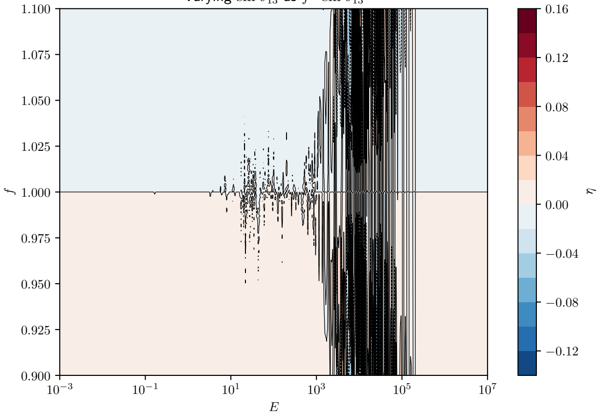
Relative P_{\mu\mu} variation for 'sun' model (passed through by 0.1 angle) Varying \sin \vartheta_{13} as f \cdot \sin \vartheta_{13}
