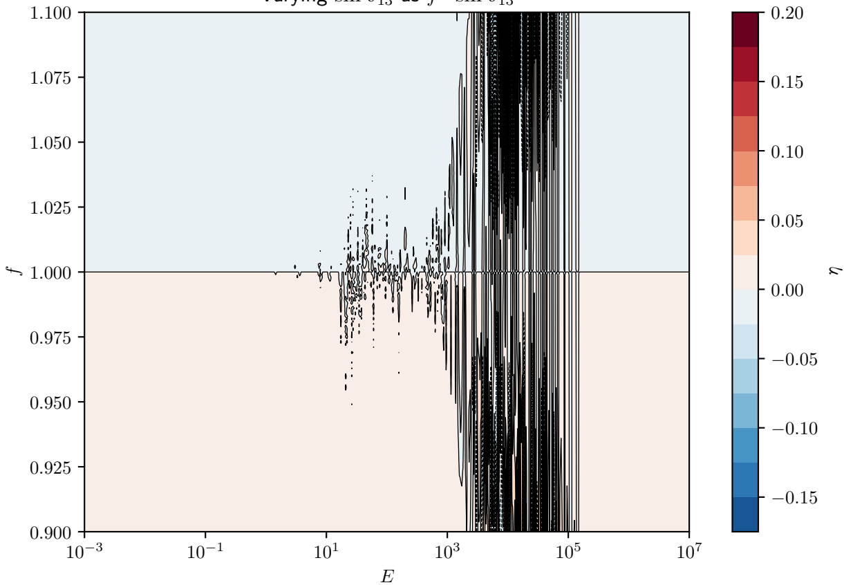
Relative P_{\mu\mu} variation for 'sun' model (passed through by 0.5 angle) Varying \sin \vartheta_{13} as f \cdot \sin \vartheta_{13}
