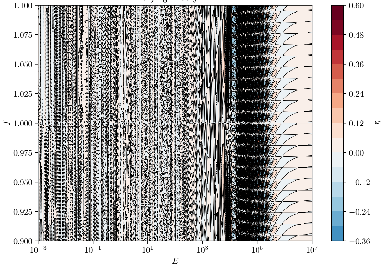
Relative P_{\text{eq}} variation for 'sun' model (passed through by 0.5 angle) Varying A as f \cdot A
