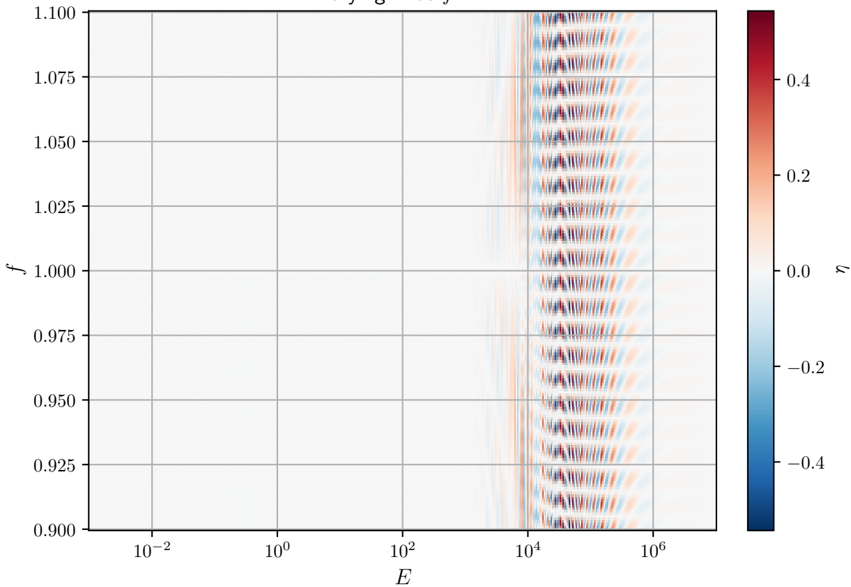
Relative P_{e\mu} variation for 'sun' model (passed through by 0.5 angle) Varying A as f \cdot A
