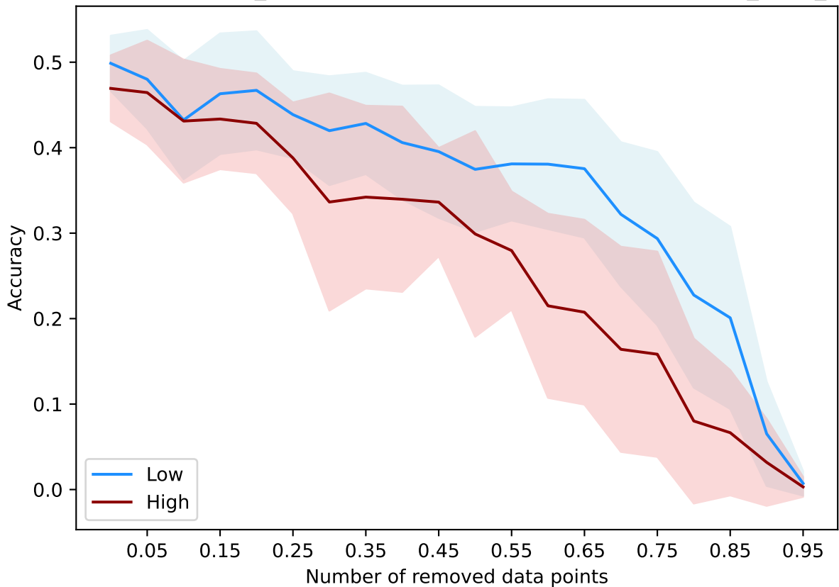
DataBanzhaf(num_models=1000) - cifar10-embeddingsworst_class_acc
