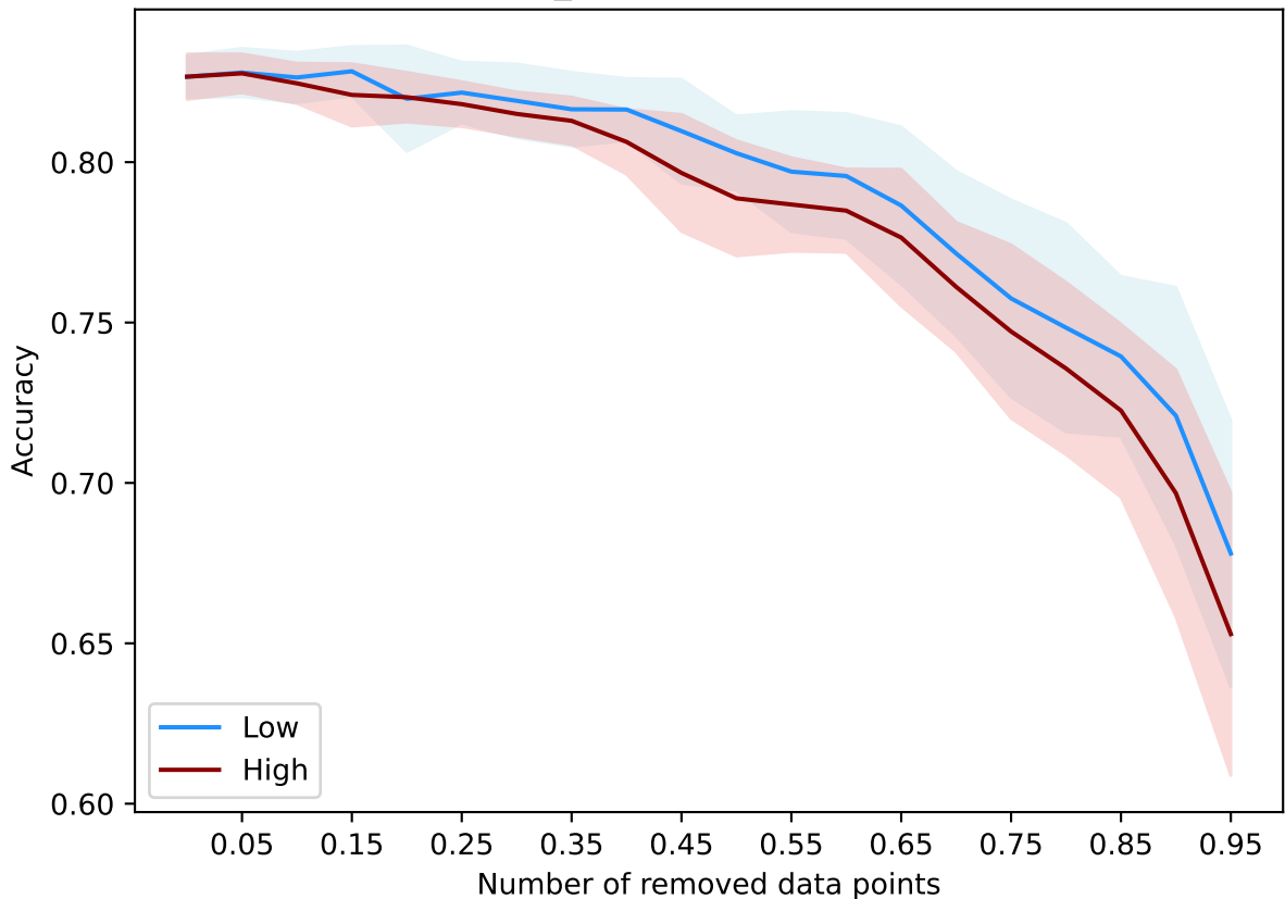
DataBanzhaf(num_models=1000) - imdb-embeddings
