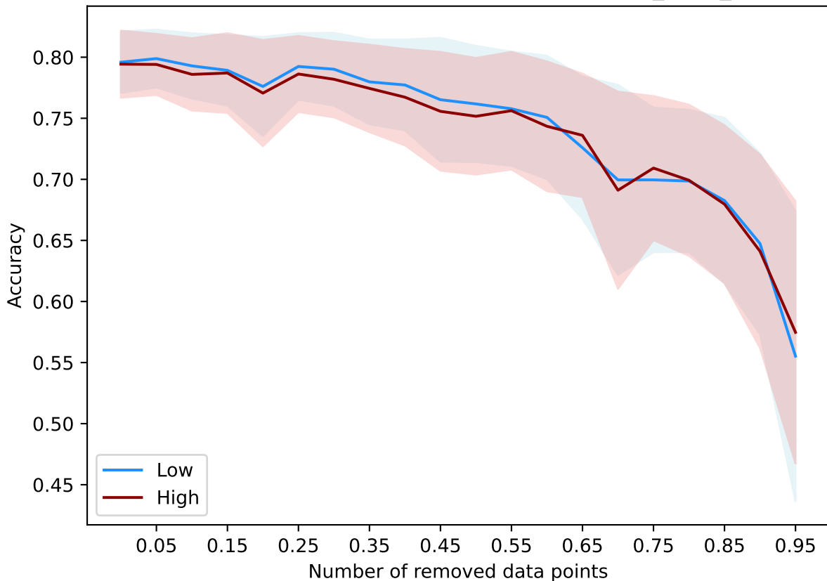
RandomEvaluator() - imdb-embeddingsworst_class_acc
