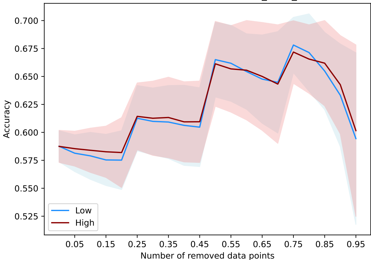
RandomEvaluator() - adultworst_class_acc
