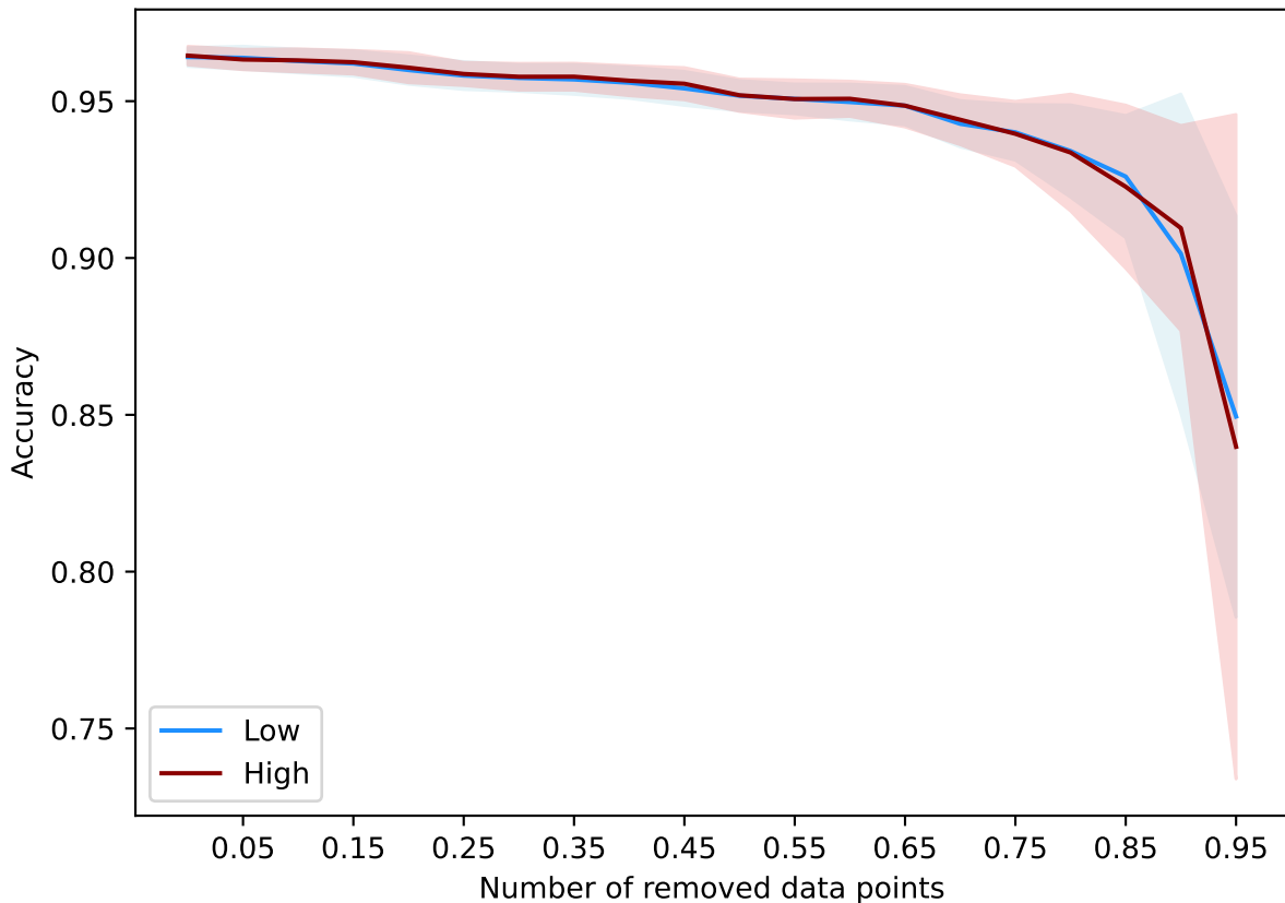
RandomEvaluator() - bbc-embeddings
