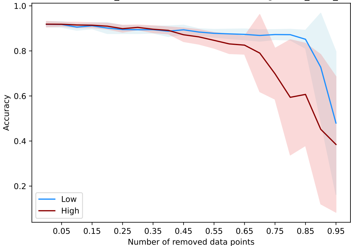
DataBanzhaf(num_models=1000) - bbc-embeddingsworst_class_acc
