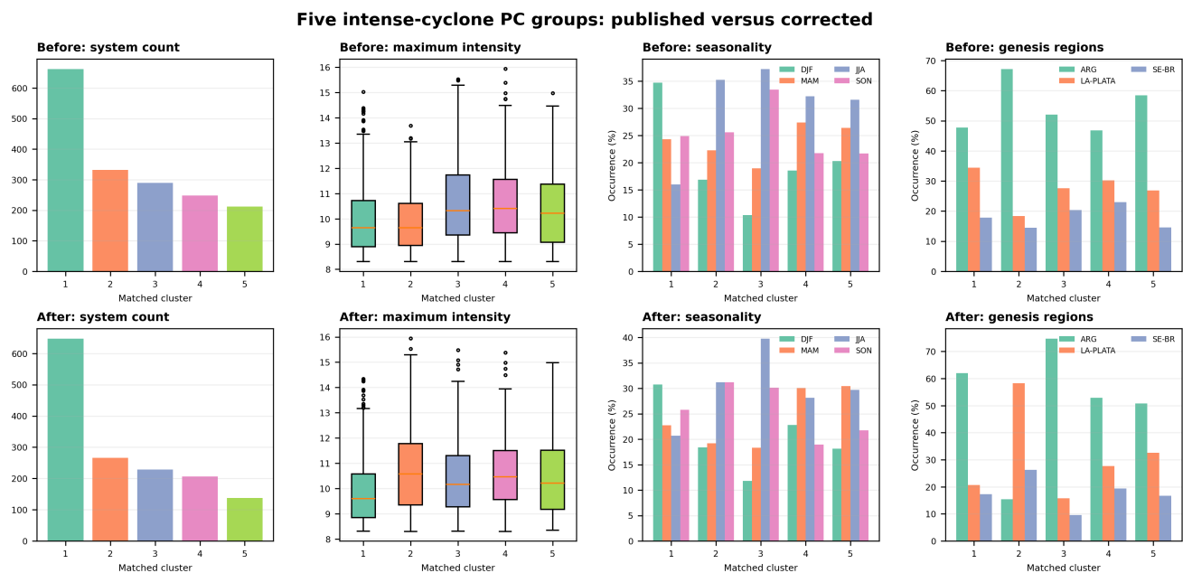
Counts, maximum intensity, seasonality and genesis regions for the five intense-cyclone PC groups.
