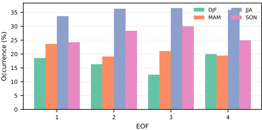
Before: seasonal occurrence - EOF(+)
