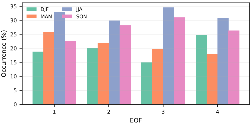
After: seasonal occurrence - EOF(+)
