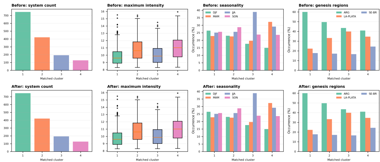
Intense-group counts, intensity, seasonality and genesis regions, before above and after below.
