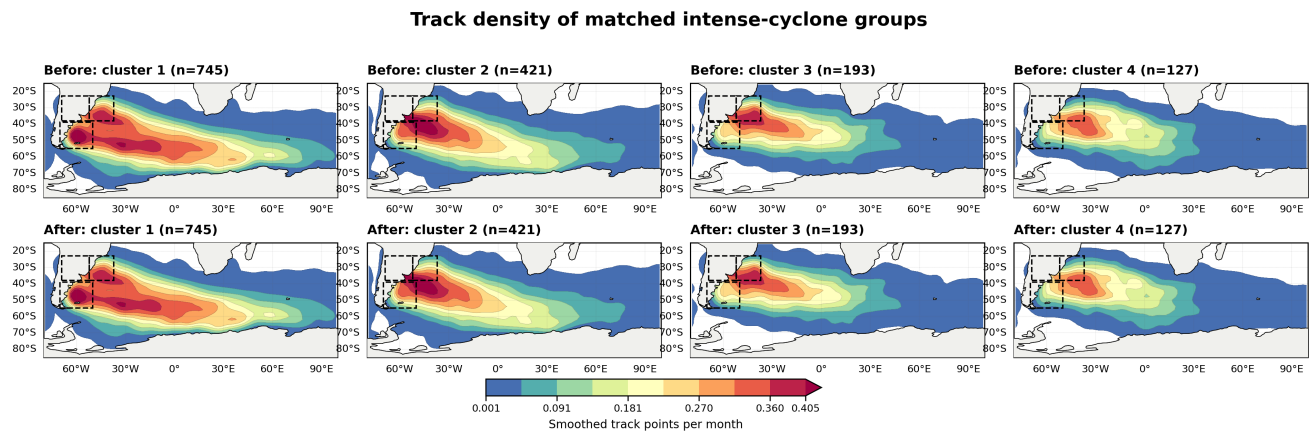
Track densities of intense-cyclone groups, before above and centroid-matched after groups below.
