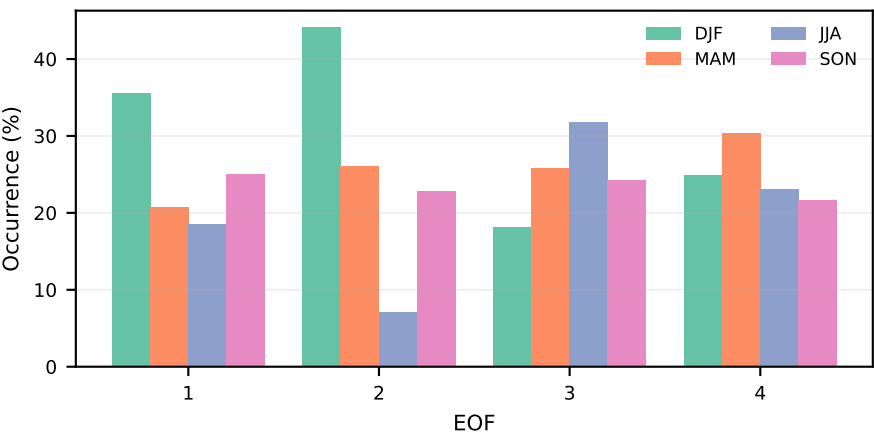
After: seasonal occurrence - EOF(-)
