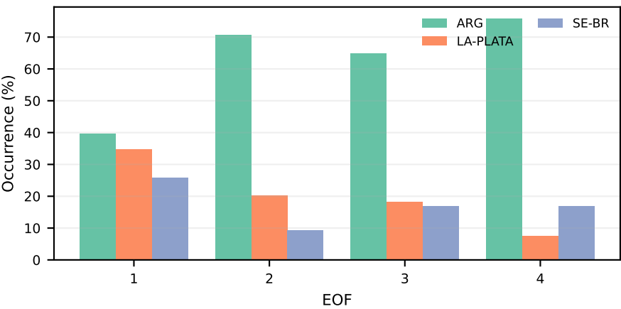
After: genesis regions - EOF(+)
