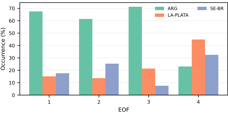
Before: genesis regions - EOF(-)
