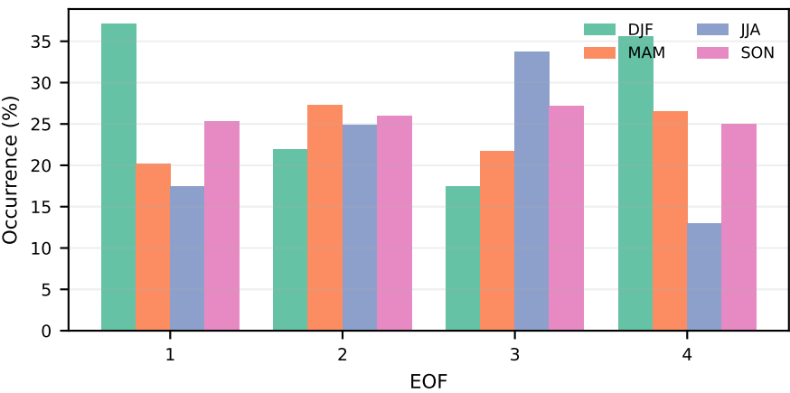
Before: seasonal occurrence - EOF(-)
