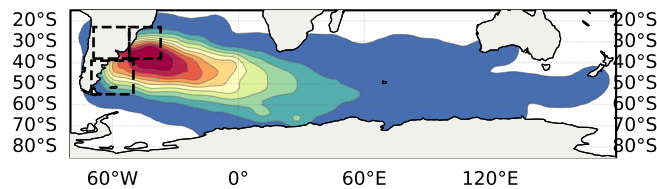
Before: EOF 1 (n=315)
