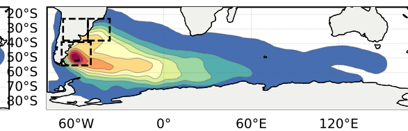
Before: EOF 2 (n=320)
