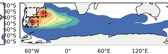
Before: EOF 3 (n=299)
