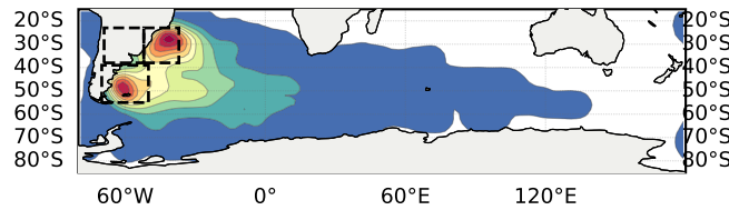
Before: EOF 1 (n=332)
