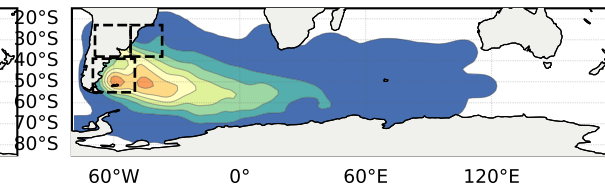
Before: EOF 3 (n=332)
