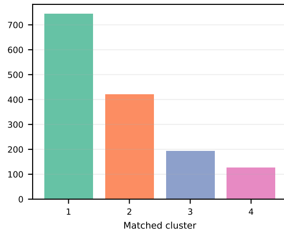
After: system count
