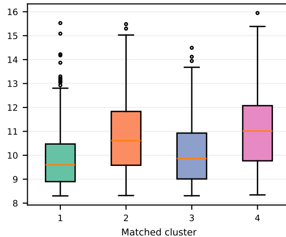
After: maximum intensity
