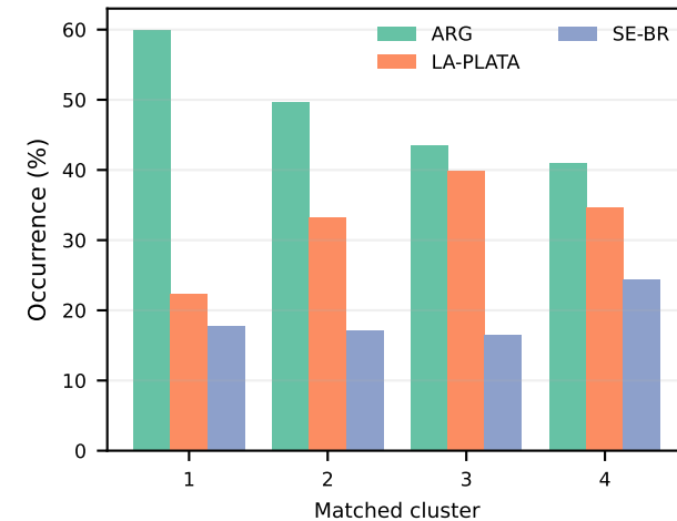
After: genesis regions
