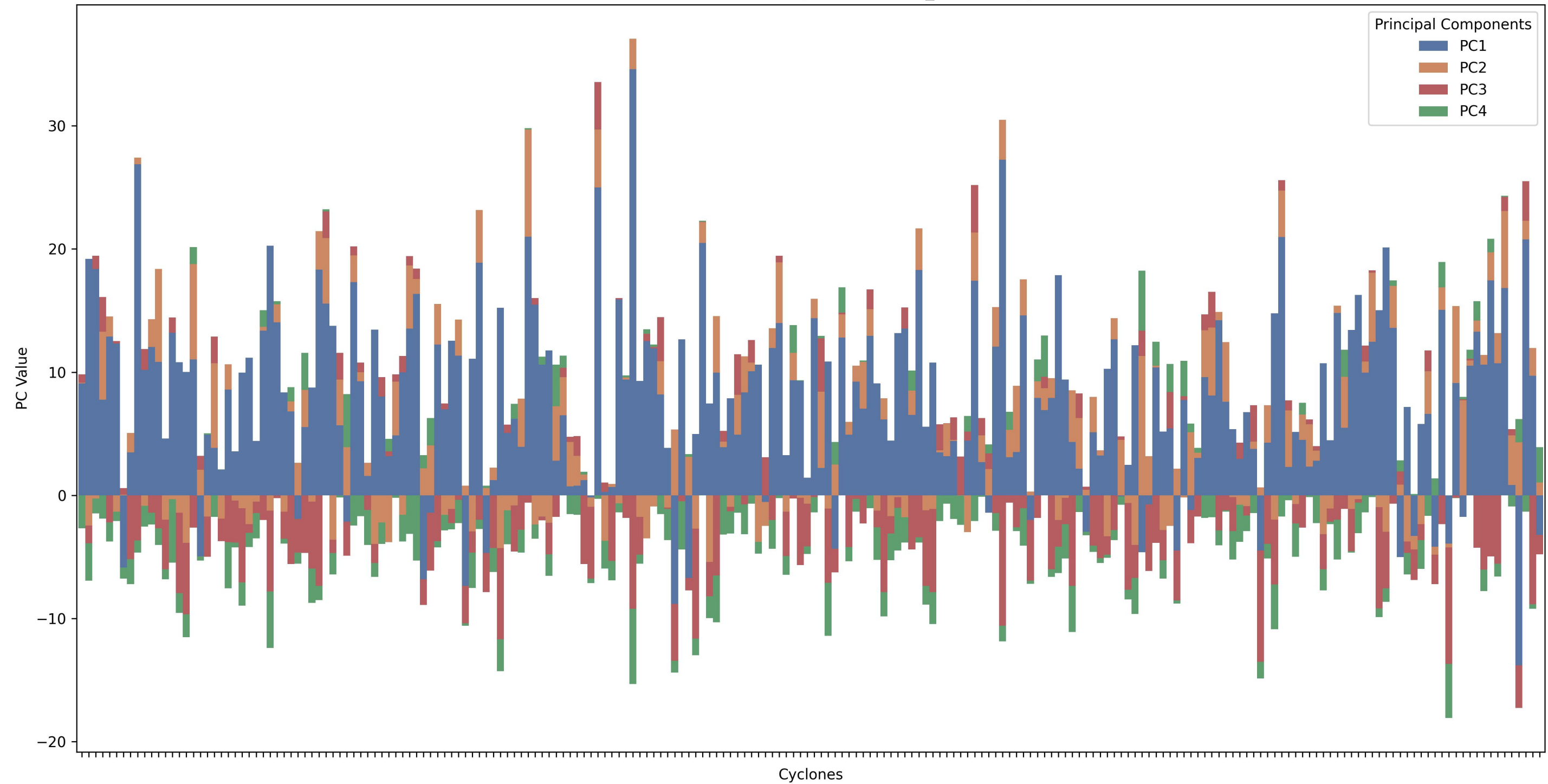
PC1 to PC4 Time Series - Cyclones with \zeta_{\text{central}} > q99
