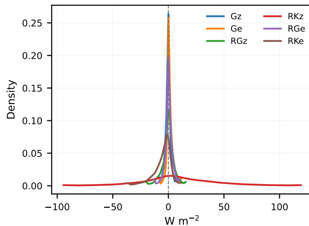
(E) Generation/residual terms
