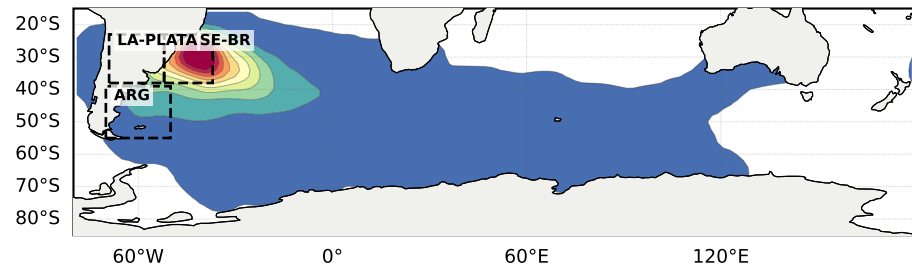
(C) EOF 3 (n=284)
