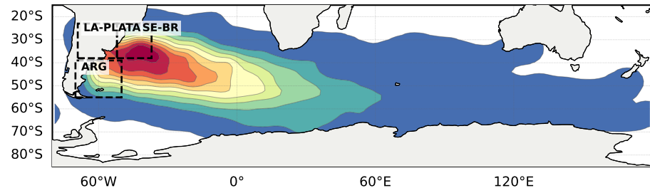
(A) EOF 1 (n=316)
