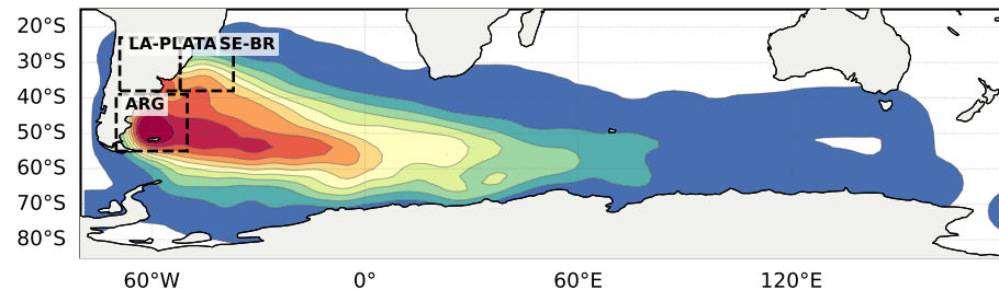
(C) EOF 3 (n=345)
