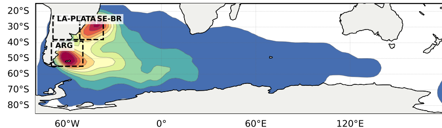
(A) EOF 1 (n=311)
