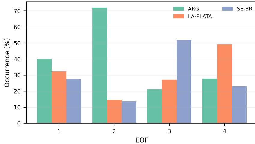
(C) Genesis proportion - EOF(-)
