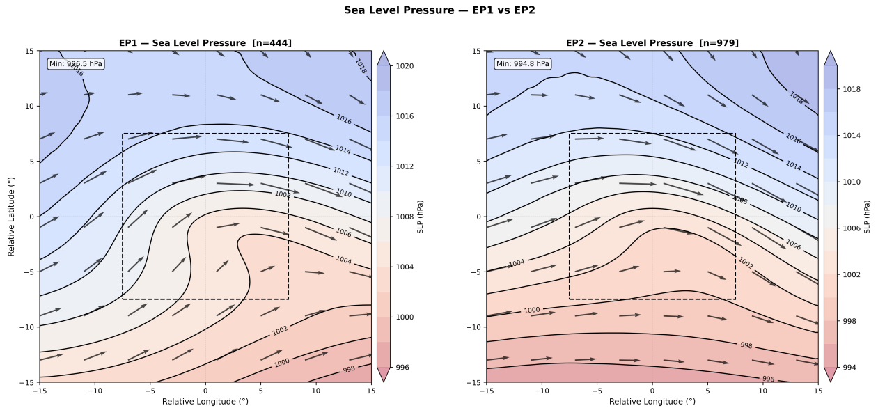
Figure 5: SLP Composite
