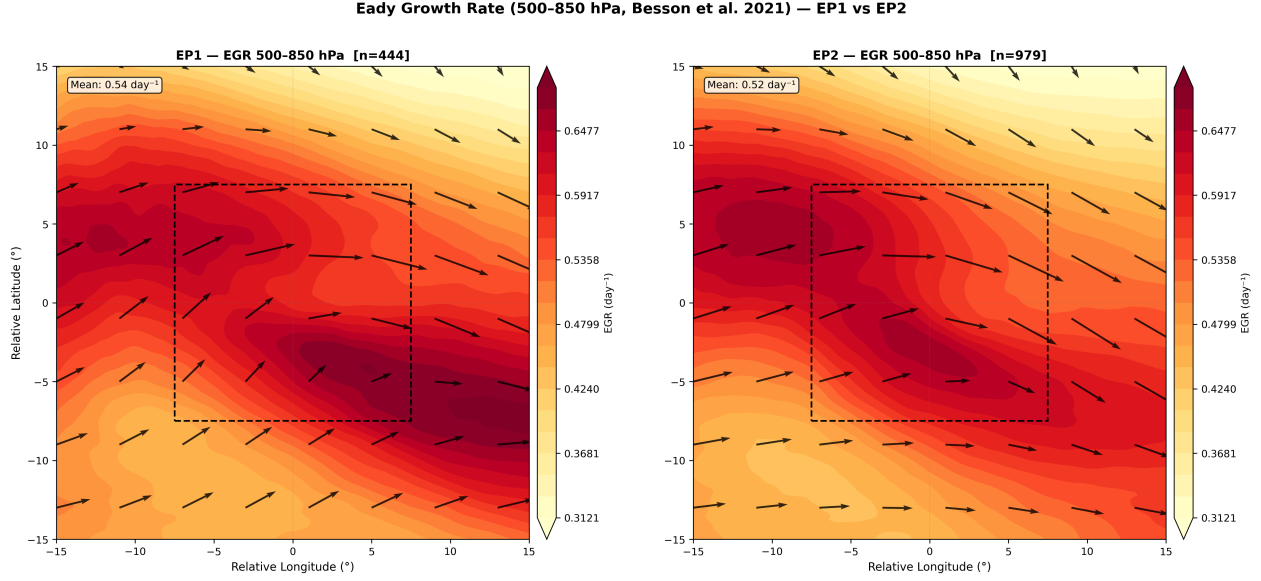
Figure 1: EGR Composite
