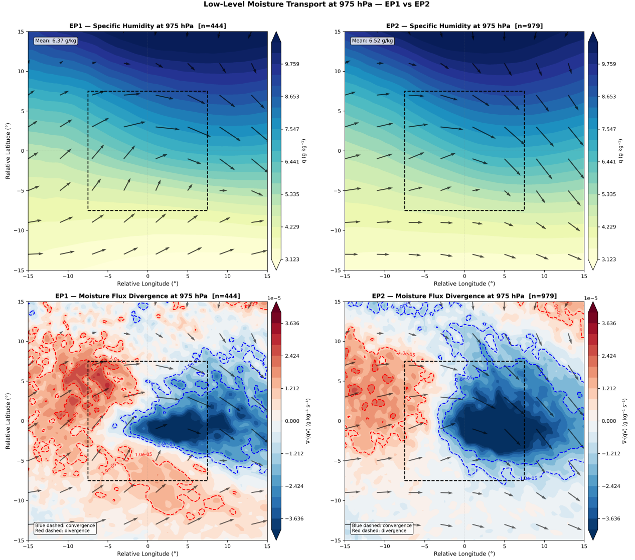
Figure 6: Moisture Composite
