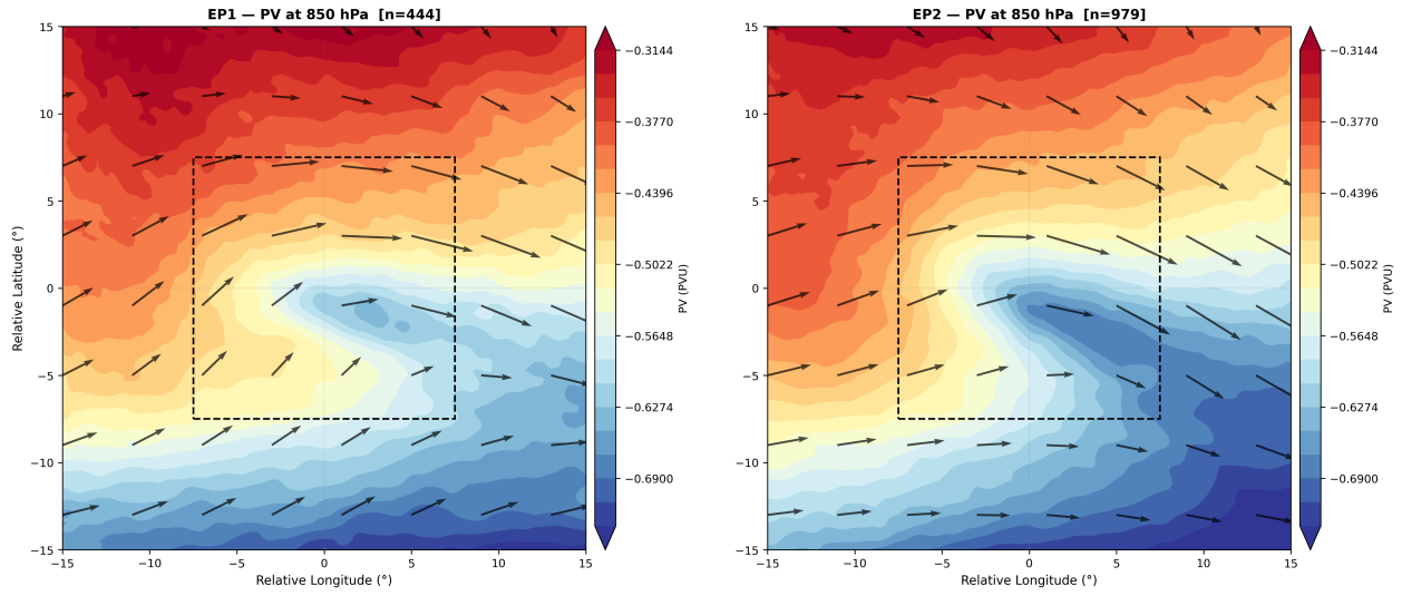
Figure 3: PV@850 Composite
