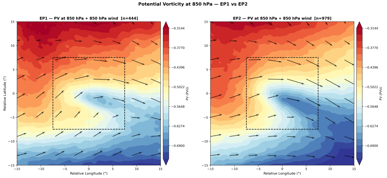
Figure 3: PV@850 Composite
