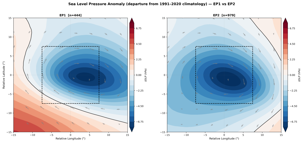
Figure 15: SLP Composite
