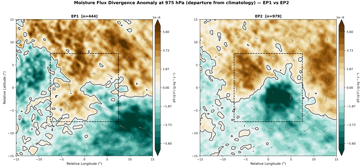
Figure 13: MFD @975 Composite
