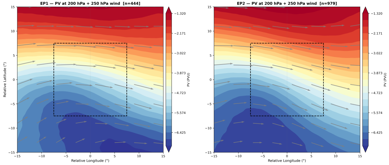
Figure 2: PV@200 Composite
