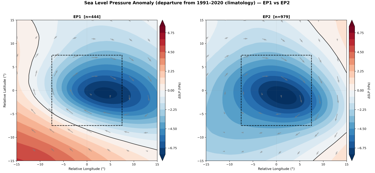
Figure 15: SLP Composite
