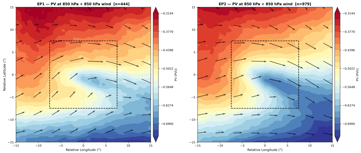
Figure 3: PV@850 Composite
