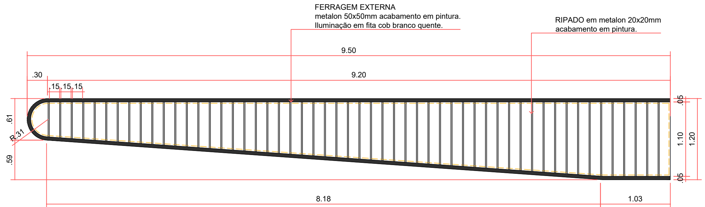
VISTA FRONTAL
