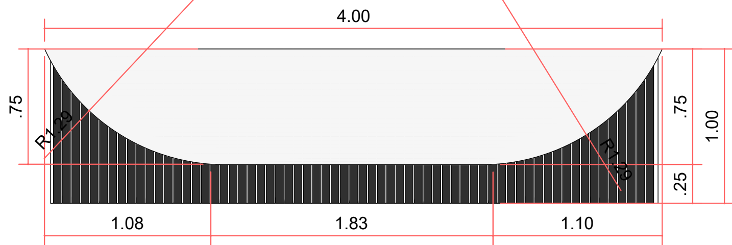
VISTA FRONTAL
