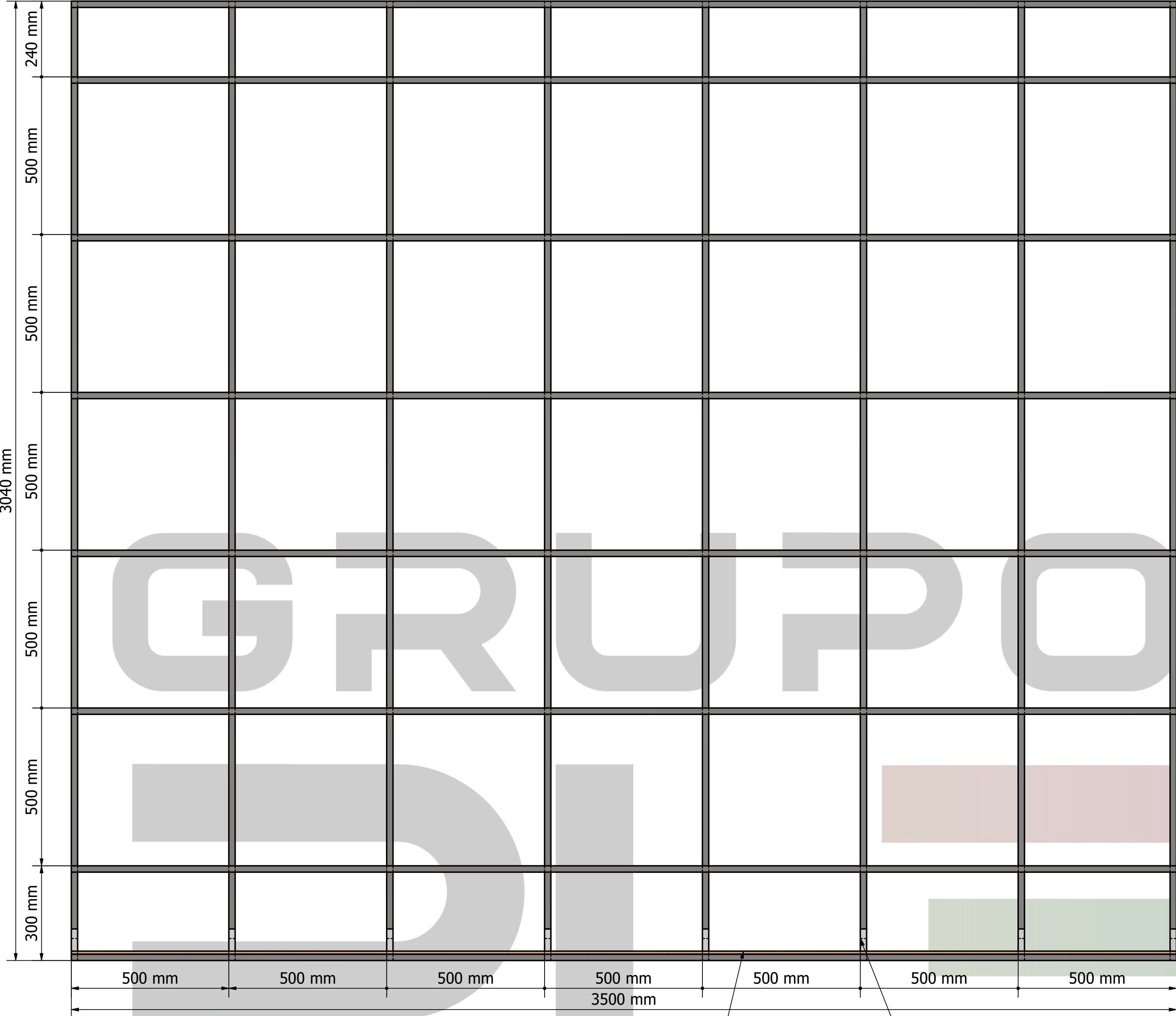
VISTA FRONTAL
