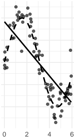
High bias (Underfit)
