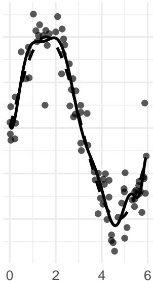
Overfit (Too complex)
