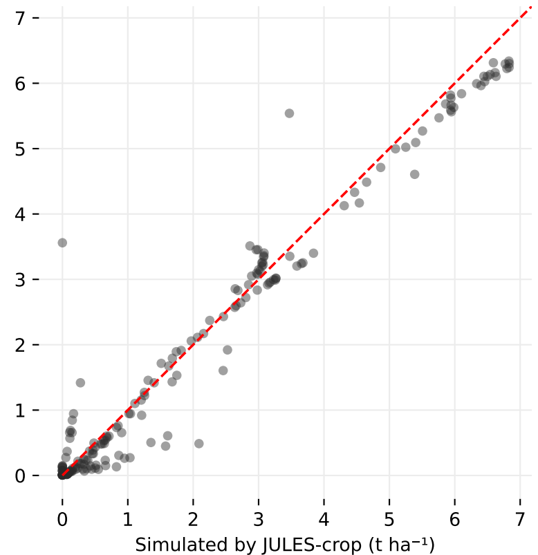
SDM ( R^2 = 0.96 , RMSE = 0.45 \text{ t ha}^{-1} )
