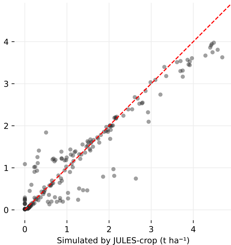
LDM ( R^2 = 0.89 , RMSE = 0.41 \text{ t ha}^{-1} )
