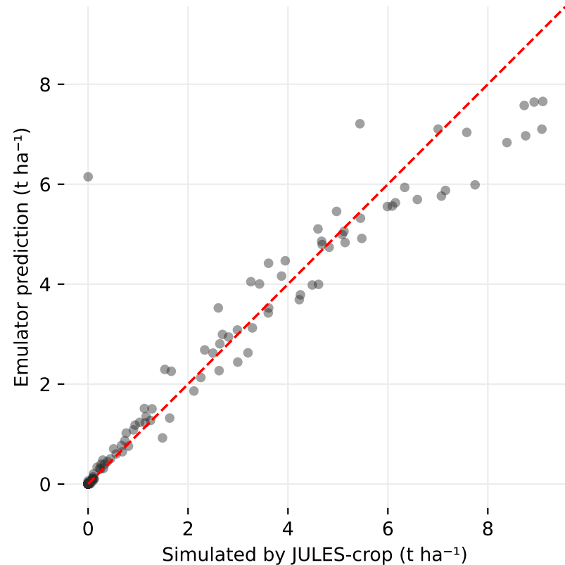
GDM ( R^2 = 0.93 , RMSE = 0.62 \text{ t ha}^{-1} )
