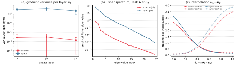
Figure 10: Mechanism measurements (10 seeds per arm). (a) Per-layer gradient variance of the Task-A loss at \theta_0 (error bars: standard deviation over seeds), (b) mean empirical Fisher spectrum of the Task-A loss at \theta_0 , (c) training losses along the linear interpolation between the two task optima (fixed 300-sample subsets).
