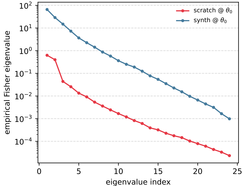
(b) Fisher spectrum, Task A at \theta_0
