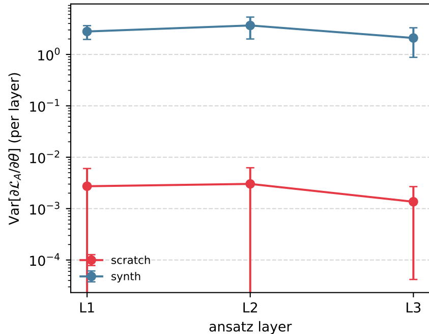
(a) gradient variance per layer, \theta_0
