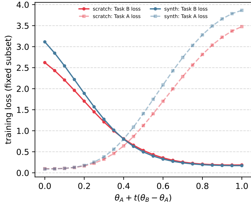
(c) interpolation \theta_A \rightarrow \theta_B
