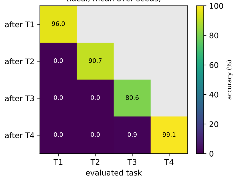
class-IL accuracy matrix — scratch (ideal, mean over seeds)
