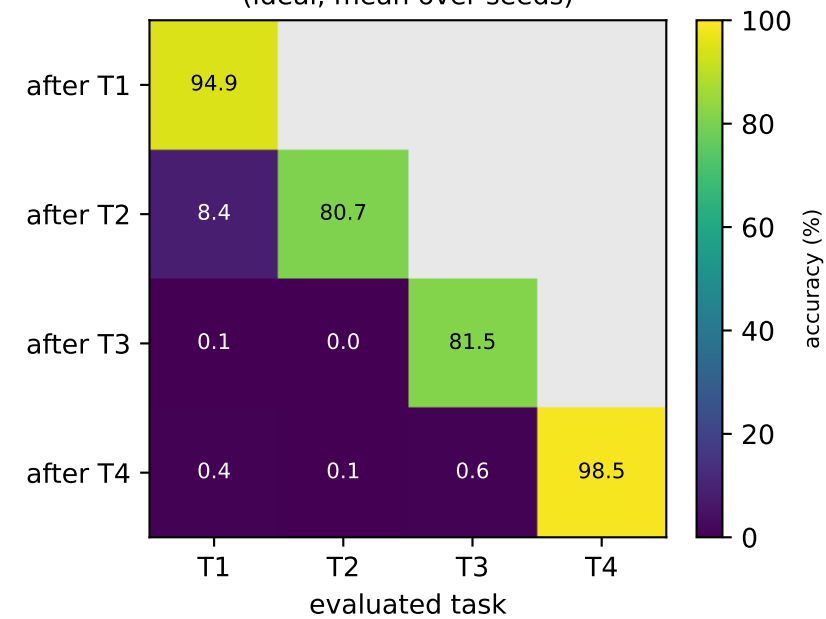
class-IL accuracy matrix — synth (ideal, mean over seeds)
