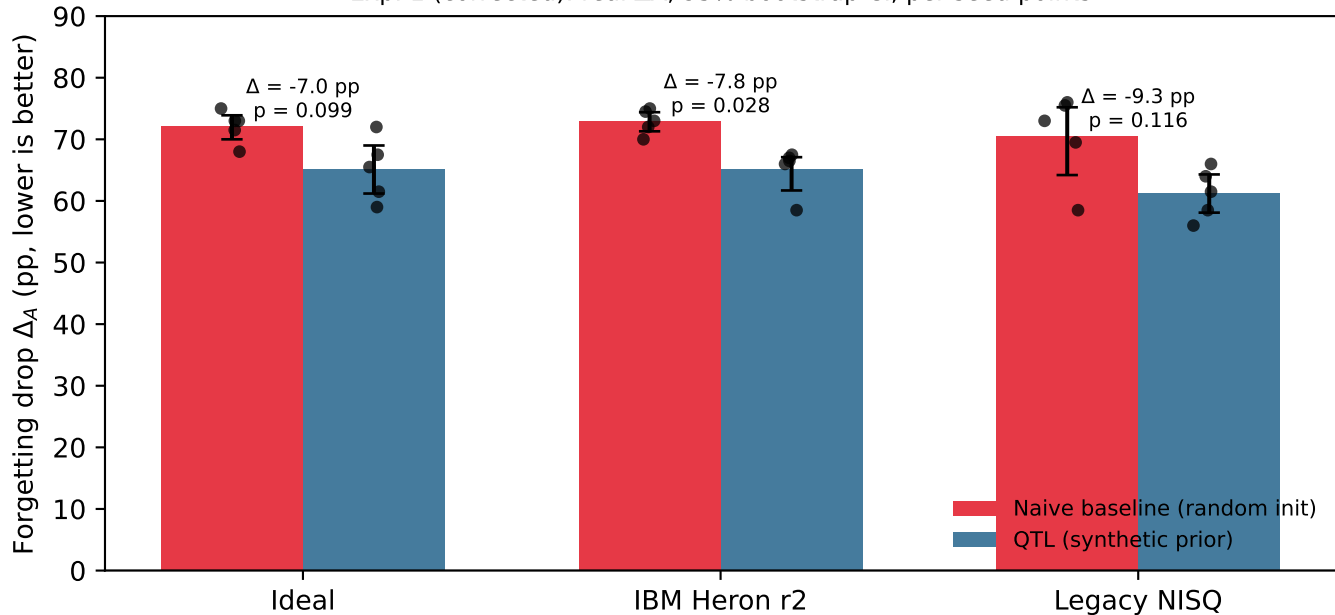
Exp. 1 (corrected): real \Delta A , 95% bootstrap CI, per-seed points
