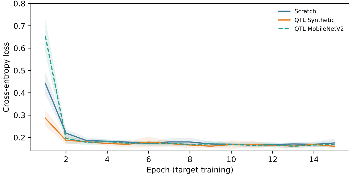
Exp. 3 corrected: real cross-entropy curves (IBM Heron r2, mean \pm SD over 5 seeds)
