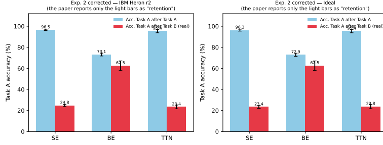
Figure 2: Experiment 2. Task A accuracy before and after the sequential exposure to Task B for each topology under the device noise profile. The gap between the two measurements is the true forgetting drop.
