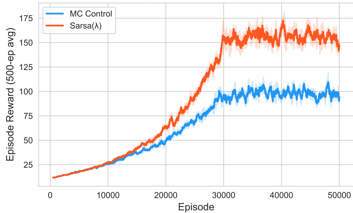
Learning Curves — Training Reward
