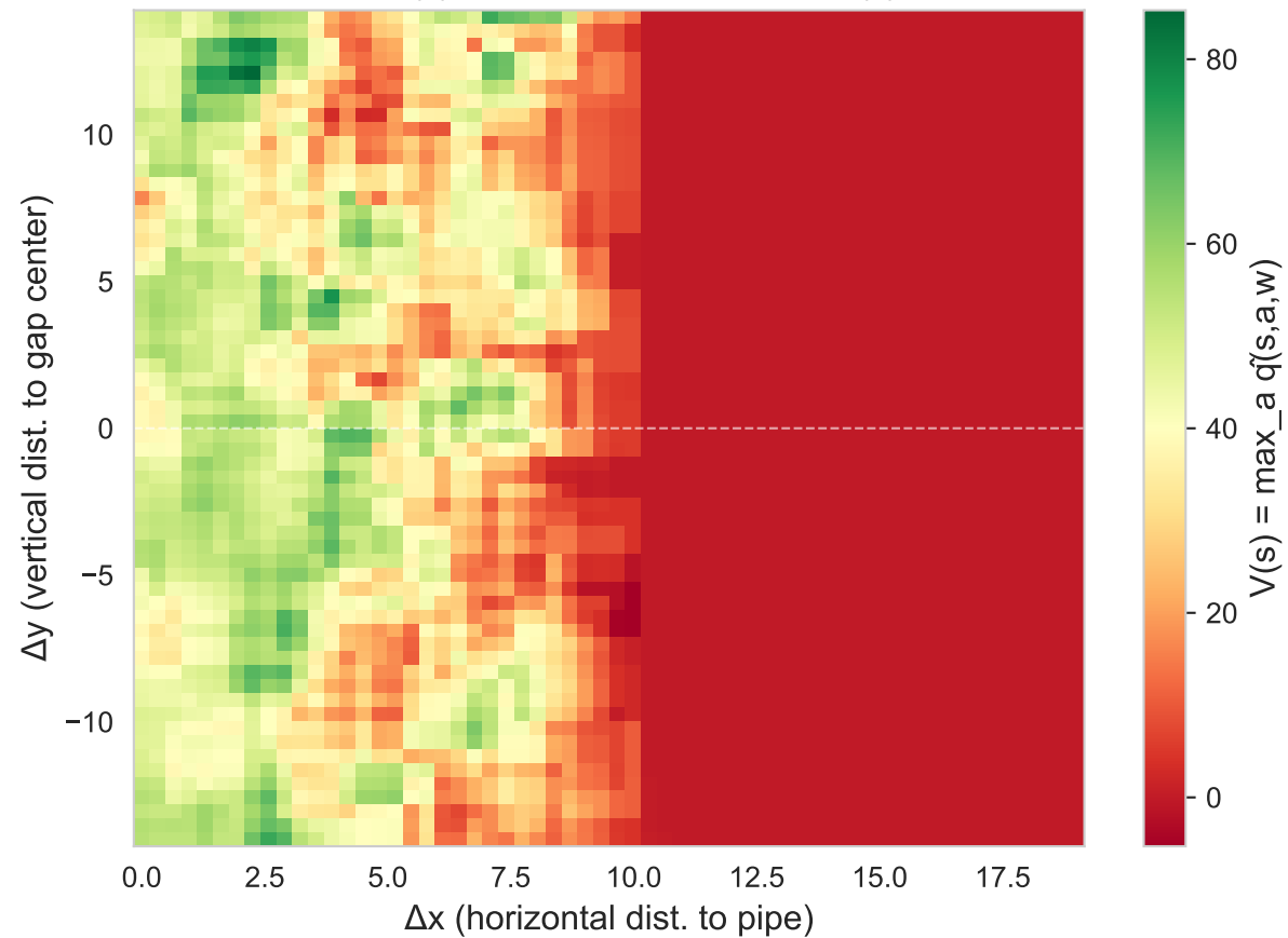
Sarsa( \lambda ) — State-Value Function V(s)
