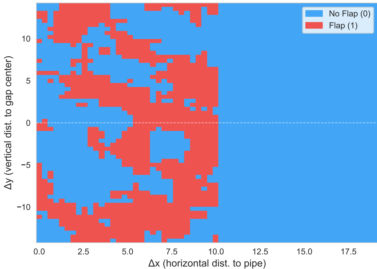
Sarsa( \lambda ) — Greedy Policy \pi(s)
