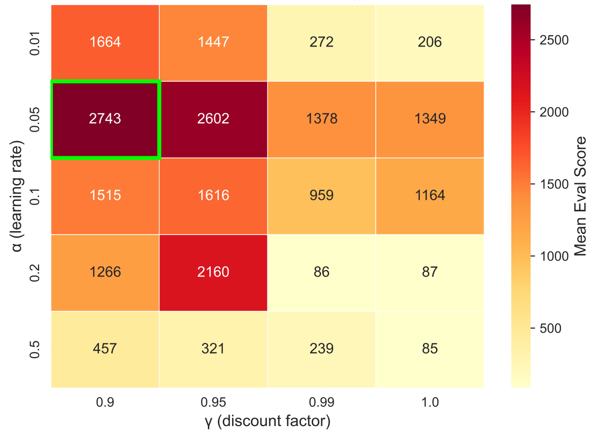
MC Control — Mean Eval Score ( \uparrow better)
