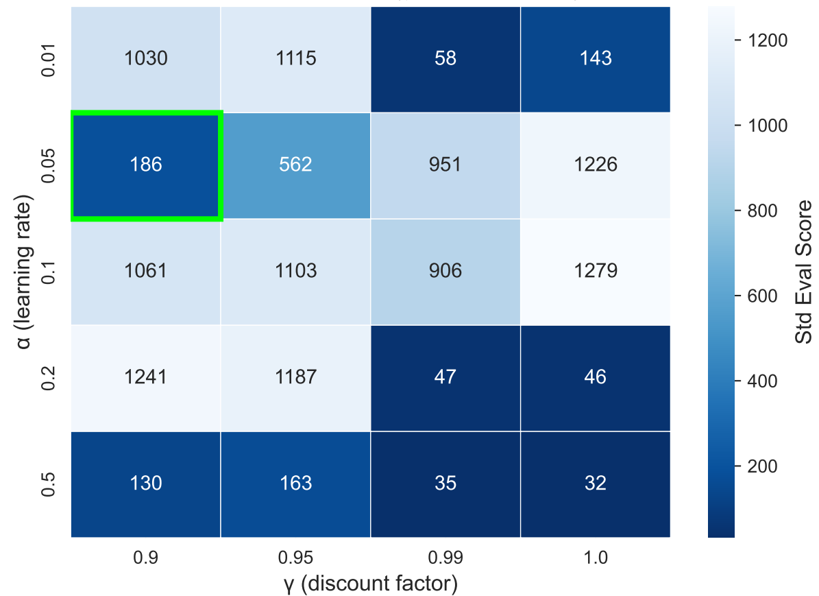
MC Control — Eval Std ( \downarrow more consistent)
